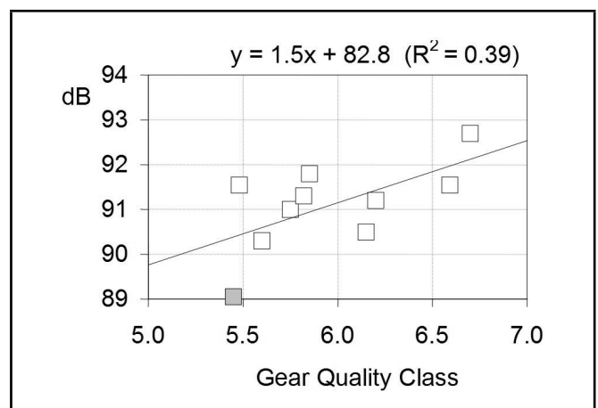
Figure 11. Effect of mean gear quality on noise level in dB at 1 m.
