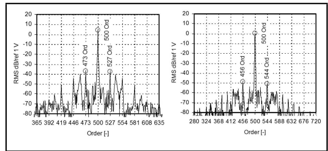
Figure 14. Frequency spectrum of phase modulated signal generated by the encoders that are attached to the secondary shaft (27-tooth gear) and the output shaft (44-tooth gear) of the gearbox shown in Fig. 3.
