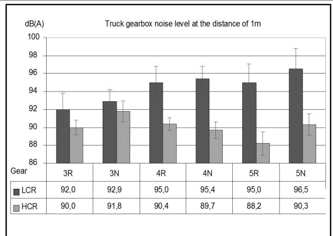
Figure 13. The gearbox overall noise level of the HCR gears in comparison with the LCR gears for 6 engaged gears important for the pass-by noise level measurement.
