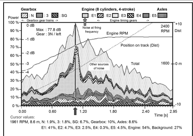
Figure 1. Truck noise sources contribution to overall pass-by noise level.
