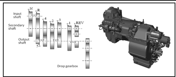
Figure 3. TATRA truck (T815-2) gearbox arrangement.
