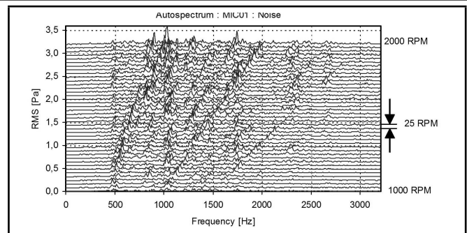
Figure 4. Running noise autospectra of the gearbox noise in RMS.
